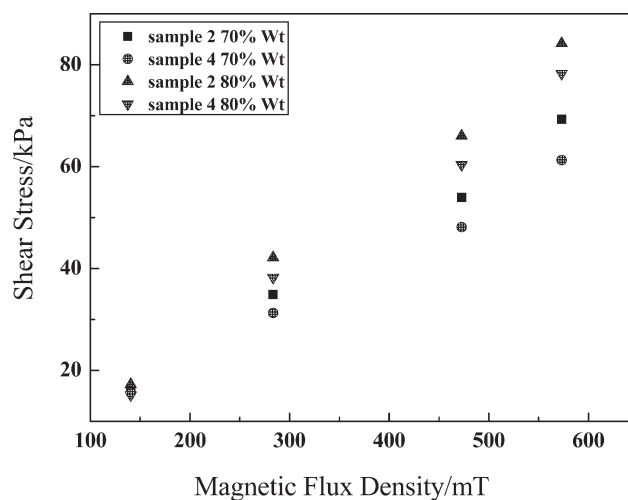
Figure 8 The dynamic shear yield stress of the samples for different molar mass of PPG in PU MRG.
