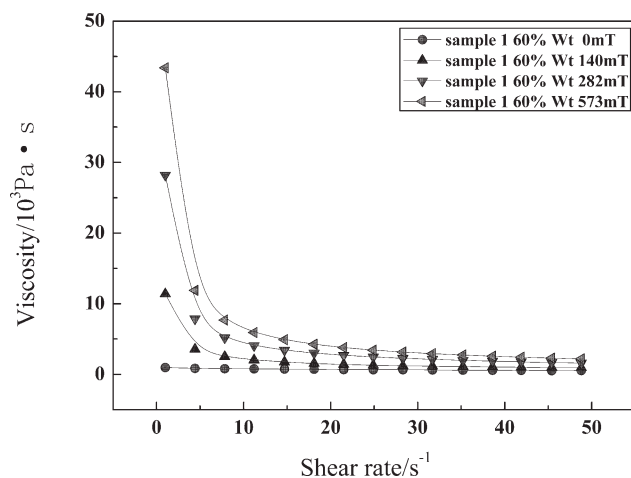
Figure 6 The viscosity of the sample1 under various magnetic fields.
