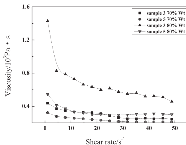
Figure 5 The viscosity of the samples for different molar mass of PPG in PU MRG.
