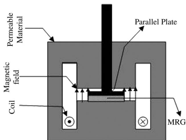
Figure 1 Principle of MR-device.
