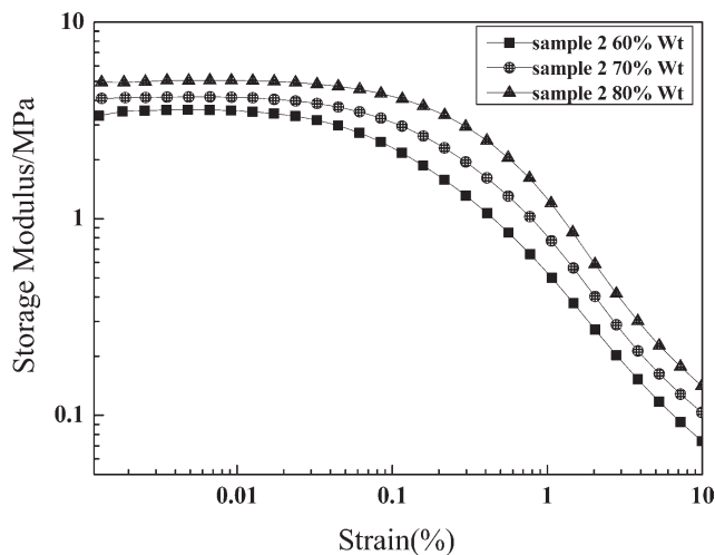
Figure 11 The storage modulus ( G' ) of the sample 2 under the same magnetic fields.
