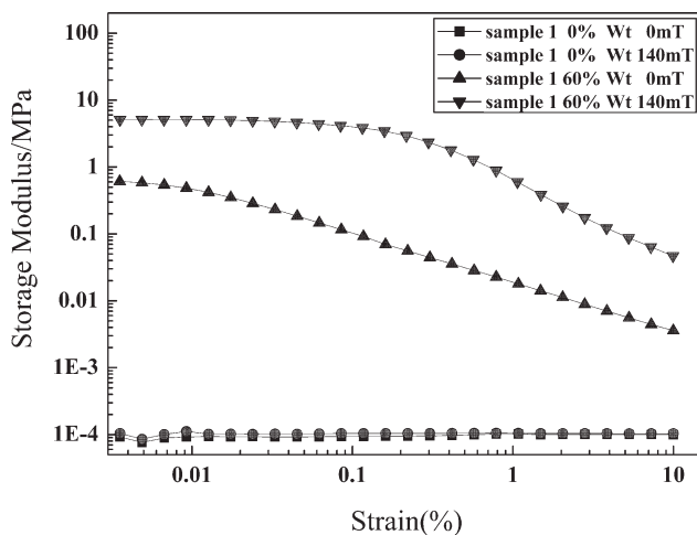
Figure 9 The storage modulus ( G' ) of the samples under different magnetic fields.
