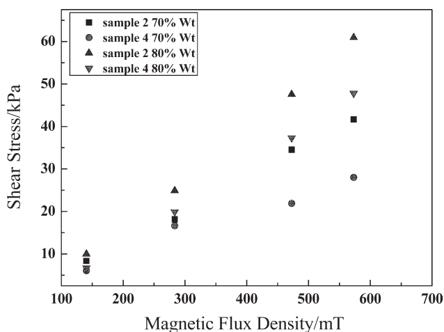
Figure 7 The static shear yield stress of the samples for different molar mass of PPG in PU MRG.
