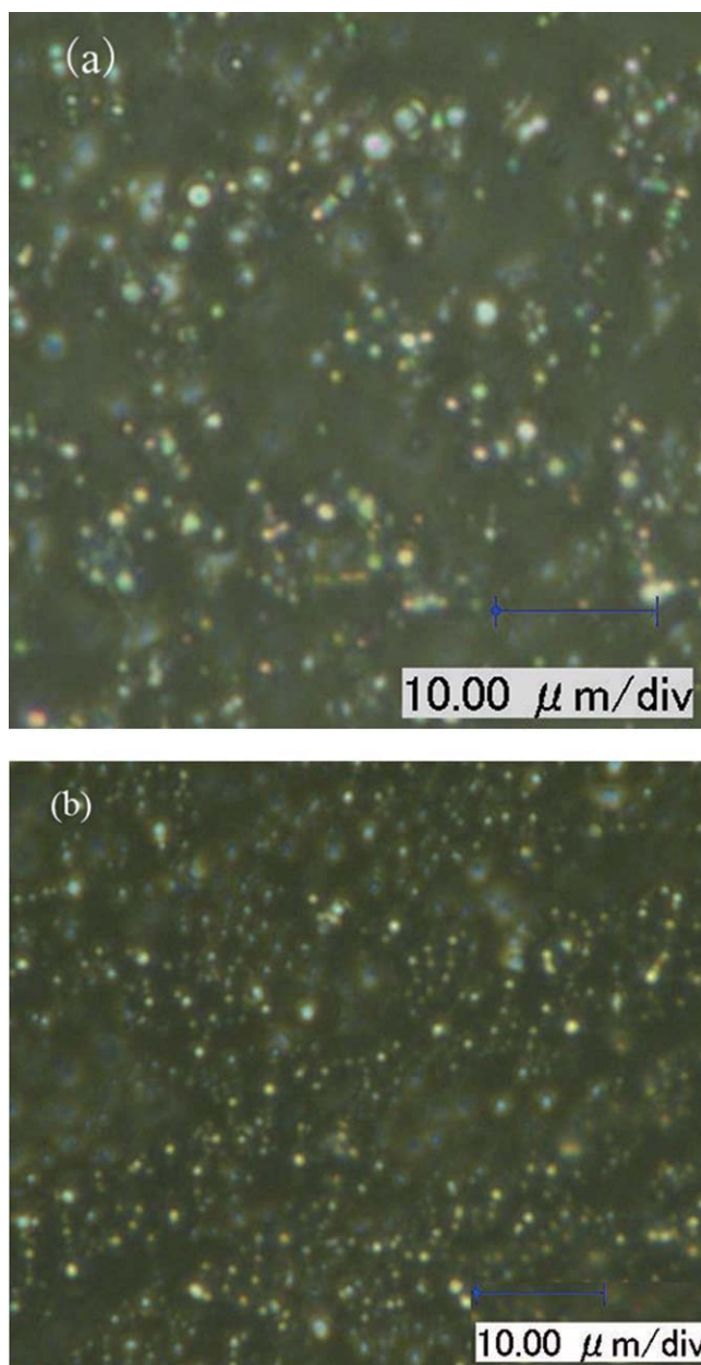
Figure 3 Optical microscopy images of the sample 4 (carbonyl iron particle: 60 wt %) observed by digital microscope: (a) 0 mT and (b) 600 mT. [Color figure can be viewed in the online issue, which is available at www.interscience.wiley.com .]
