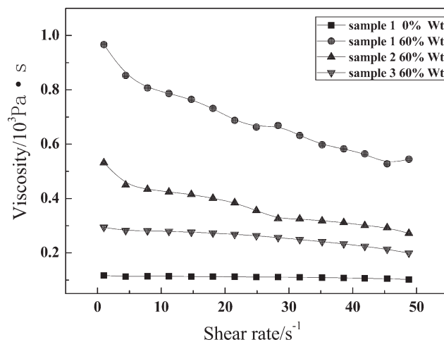
Figure 4 The viscosity of the samples for different reaction molar ratio in PU MRG.
