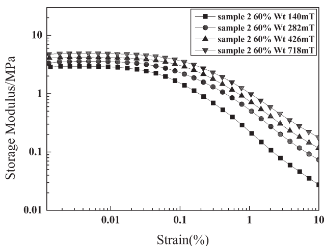
Figure 10 The storage modulus ( G' ) of the sample 2 under various magnetic fields.
